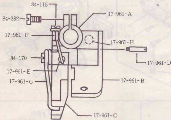
Presser foot 17-9610-1
