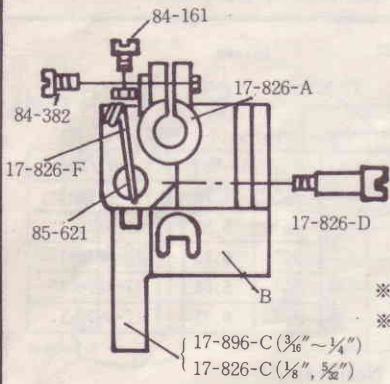
Presser foot (2 Needles)
