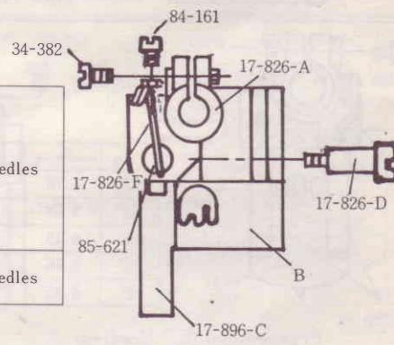
Presser foot (3 Needles)
